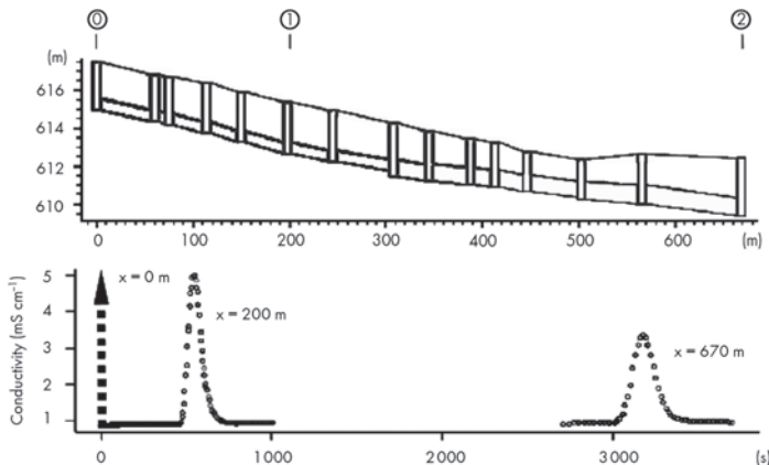
Figure 2: (Top) Longitudinal profile of a sewer section. ① = dosing point of tracer (slug injection), ① = first monitoring point (outside the initial zone), ② = second measuring point at the end of the reach. (Bottom) Tracer curves at dosing and monitoring stations. From Rieckermann et al. (2005a).
